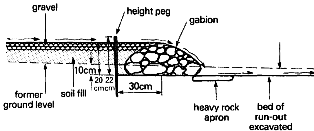
Figure 47. Construction of gabion.
