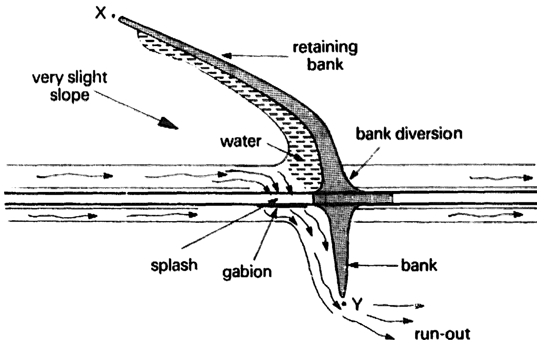
Figure 52. Diagonal splash.
