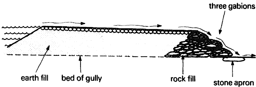
(b). Cross-section.
