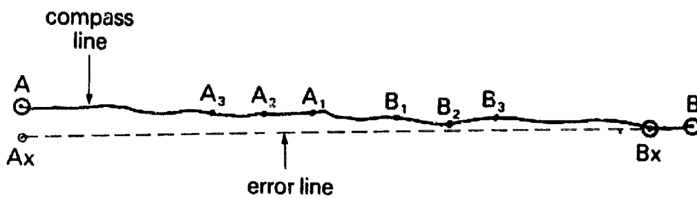
(b). Plotting the traverse.
