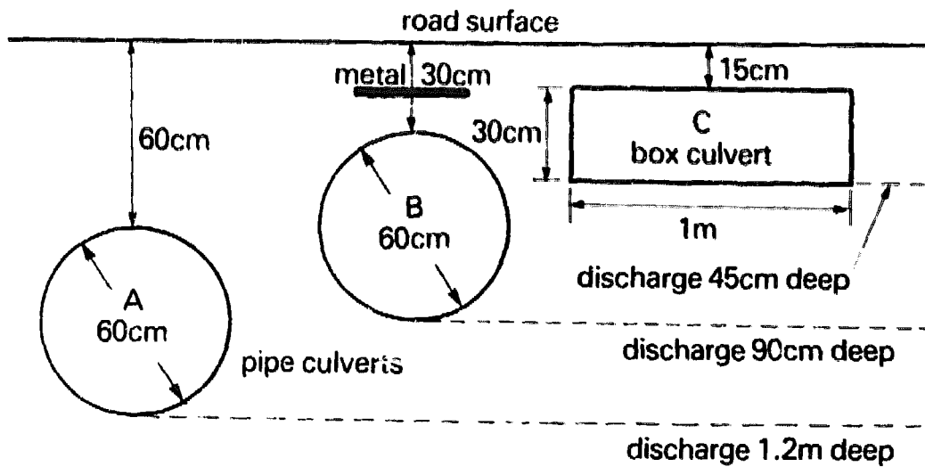
Figure 28. Methods of reducing depth of discharge.
