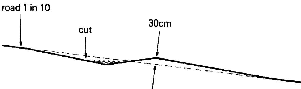
Figure 15(c). Correct bank on slope.
