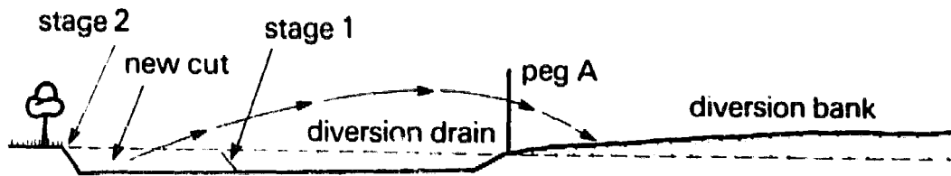
(b). Cross-section.
