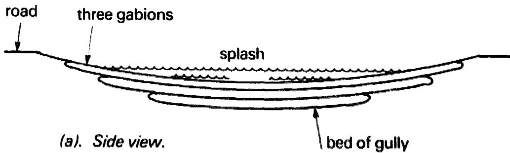
Figure 50. Splashes to be sited on straights.
