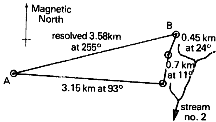
(b). Plotting the traverse.
