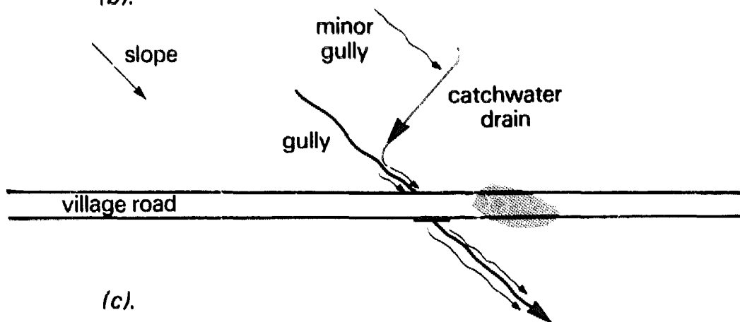
Figure 30. Catchwater drains.
