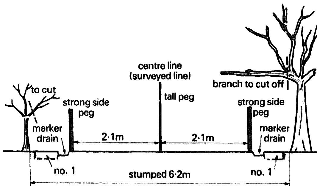
Figure 35(a). Clearing, stumping and marker drains.
