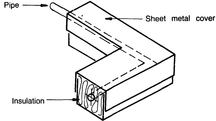
Pipe fixation with insulation
