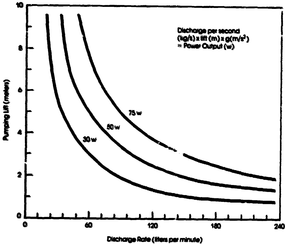
Figure B-1 Water Discharge Versus Depth
