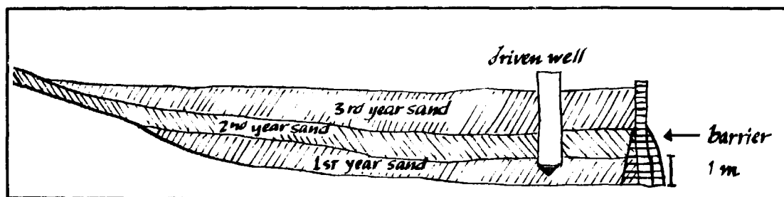
Figure 17. Cross Section of Sand Reservoir
