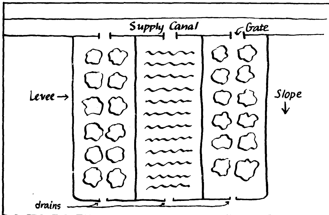
Figure 26. Border Irrigation
