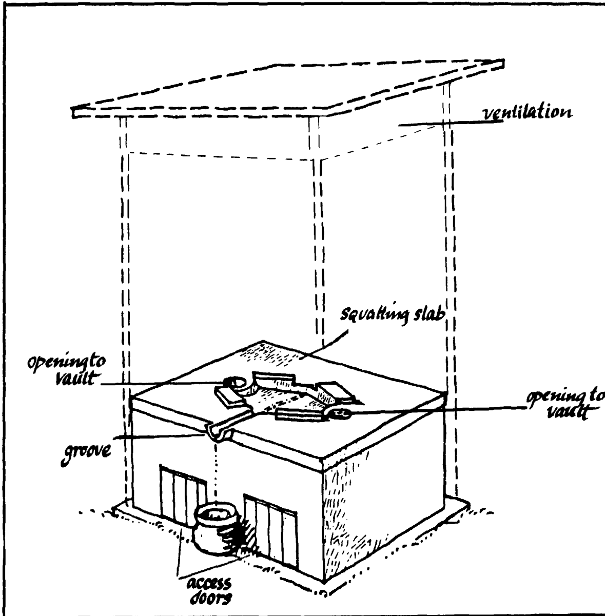
Figure 22. Double Vault Composting Latrine (after UNICEF News)
