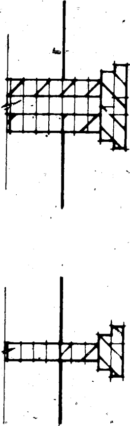
Alternative brick footing details. Scale: 1/2" to 1'-0"
