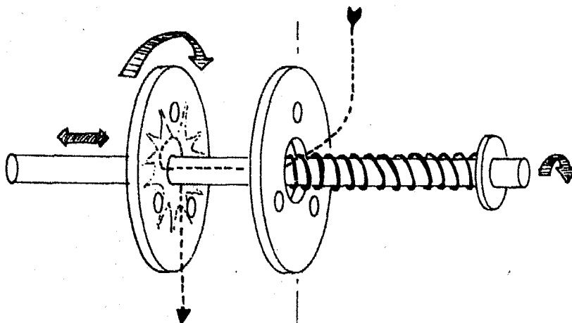
Fig. 35: Grinding principle of the Moulis grinding unit and of the locally constructible grinding unit
