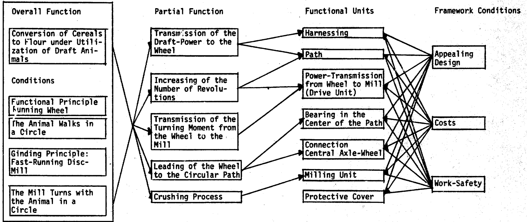
Fig. 12: Functional diagram of the animal powered mill
