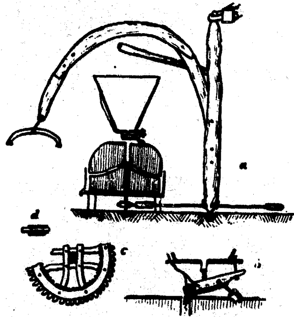
Fig. 4: Sketch of a traditional animal-powered mill from Hammamet, Tunisia
