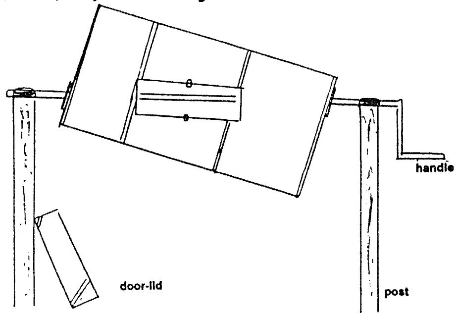
Fig. 61. Another mounting for a clean 50 gallon oil drum requires a specially fabricated locking door
