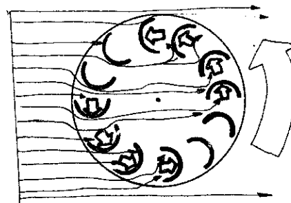
Turbine multipale
